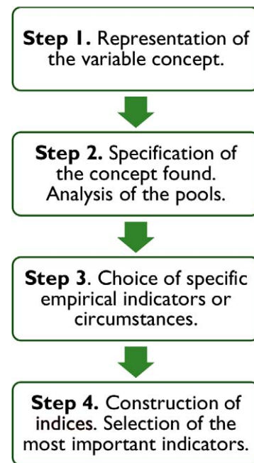
Graph 1. Procedure for variable operationalisation.
